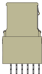
STAND-OFF, SHIELD F PIN SIDE 71-B25V-120-11XX
