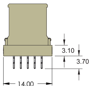
STAND-OFF, NO SHIELD 71-B25V-010-11XX
