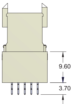
STAND-OFF, NO SHIELD 71-AB25V-020-11-XX
