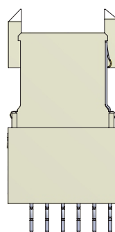
STAND-OFF, SHIELD F PIN SIDE 71-AB25V-120-11XX
