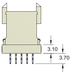
STAND-OFF, NO SHIELD 71-AB19V-010-11XX
