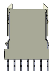
STAND-OFF, SHIELD BOTH SIDE 71-A25V-310-11XX
