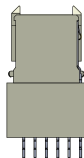
STAND-OFF, SHIELD F PIN SIDE 71-A25V-120-11XX
