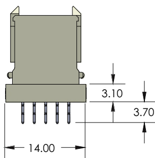
STAND-OFF, NO SHIELD 71-A25V-010-11XX
