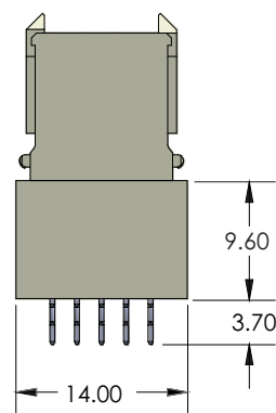
STAND-OFF, NO SHIELD 71-A25V-020-11-XX
