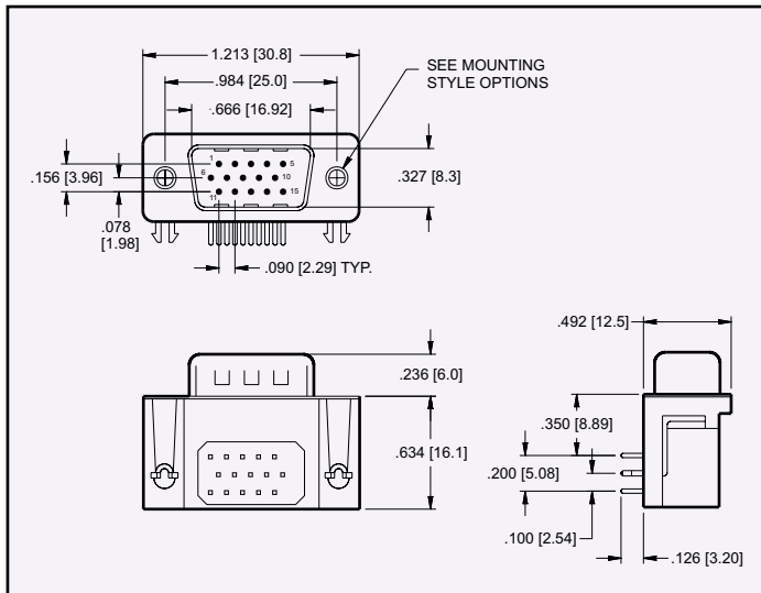
PLUG
